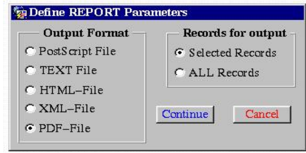
Figure 5: Report Generation System (RGS) of the GUI.
