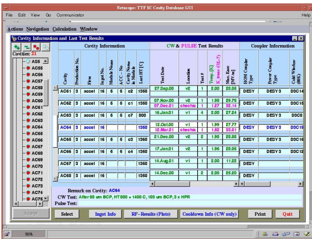
Figure 4: Results of last cw and pulsed tests of selected cavities from Summary of Last RF Tests in the GUI. A group of cavities can be selected.
