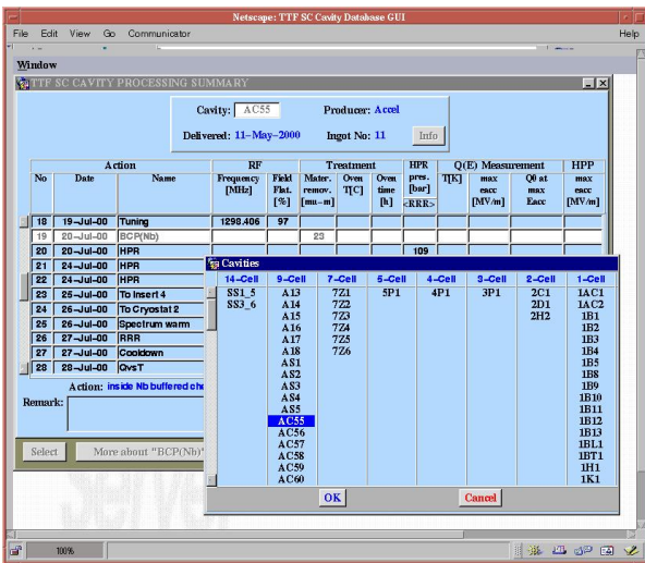
Figure 3: Summary information on preparations and tests performed on cavities in chronological order from Summary of Works/Cavity in the GUI. A specific cavity has to be selected from the list.
