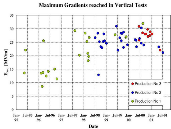
Figure 6: Maximum gradients reached in vertical tests. It is provided by MS EXCEL based on the ASCII file generated by the RGS called from Summary of Last RF Tests in the GUI.
