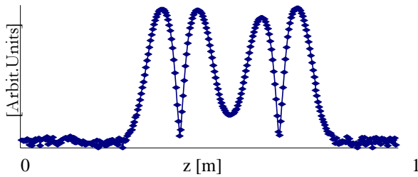
Figure 6: Measured field profile of the accelerating mode (after tuning).
