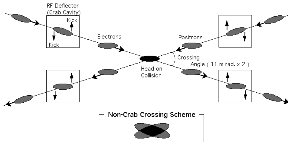
Figure 1: Crab crossing scheme for the KEKB.
