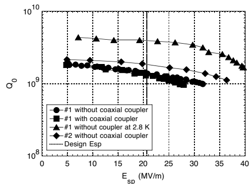
Figure 4: Performance of full-scale superconducting crab cavities with various configuration and at different temperature.
