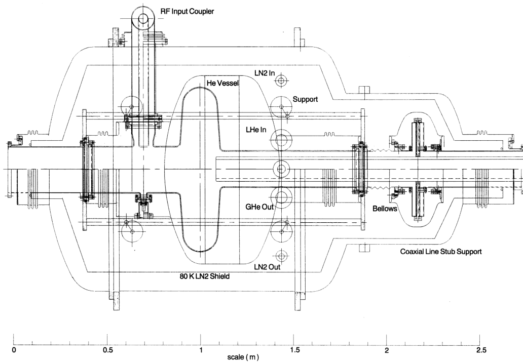
Figure 6: Cryostat design for crab cavity seen from the top.
