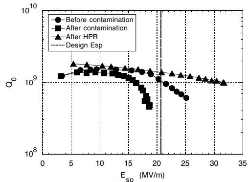
Figure 5: Effect of high pressure ultrapure water rinsing.
