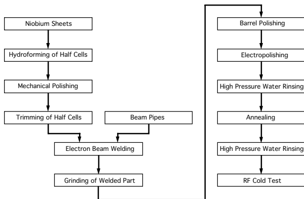
Figure 3: Fabrication and surface preparation procedure.
