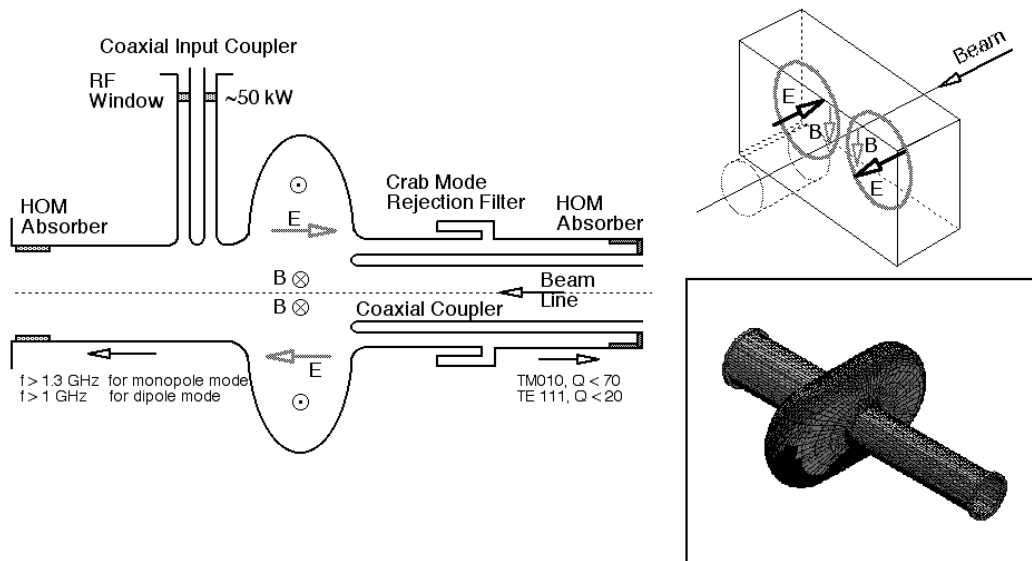
Figure 2: Concept of the squashed-cell crab cavity.
